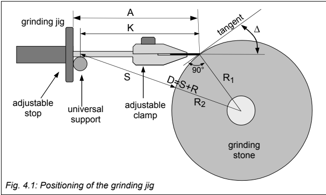
Fig. 4.1: Positioning of the grinding jig
