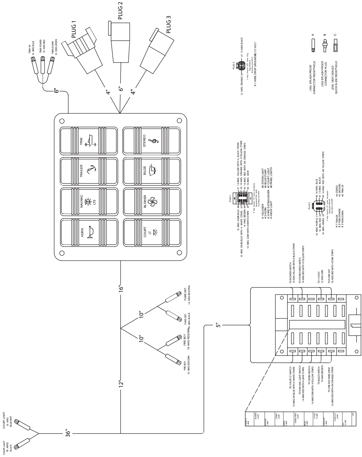
SWITCH PANEL WIRING INFORMATION (FIG. 9.1)
