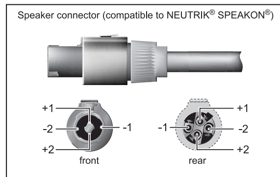
Fig. 4.1: Neutrik® Speakon®-compatible connectors
