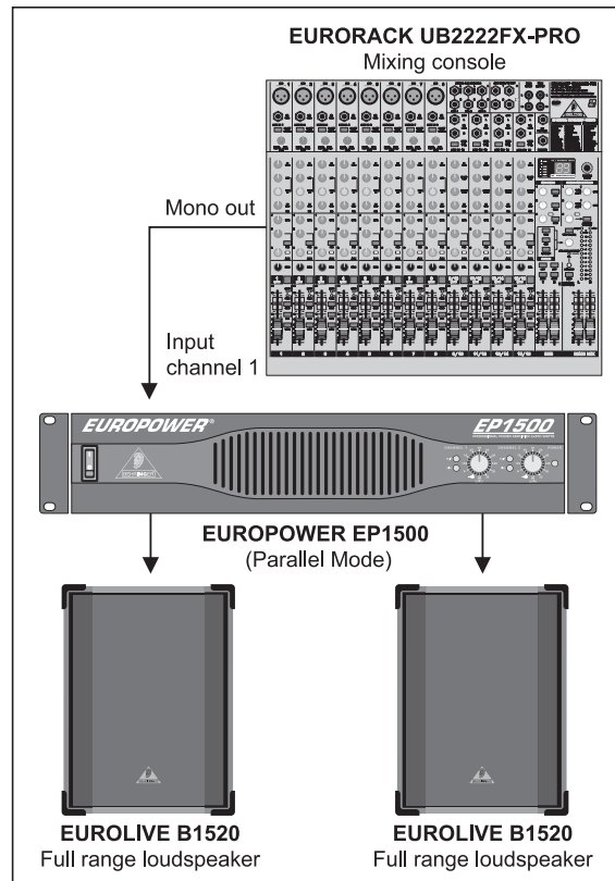
Fig. 3.3: Parallel operation
