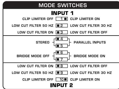
Fig. 3.2: DIP switch positions for 2-channel operation
