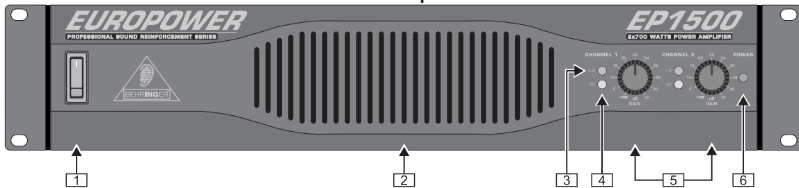
Fig. 2.1: Front panel control elements
