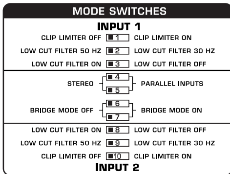
Fig. 2.3: DIP-switches
