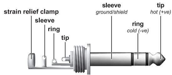
Fig. 4.5: 1/4" TRS connector
