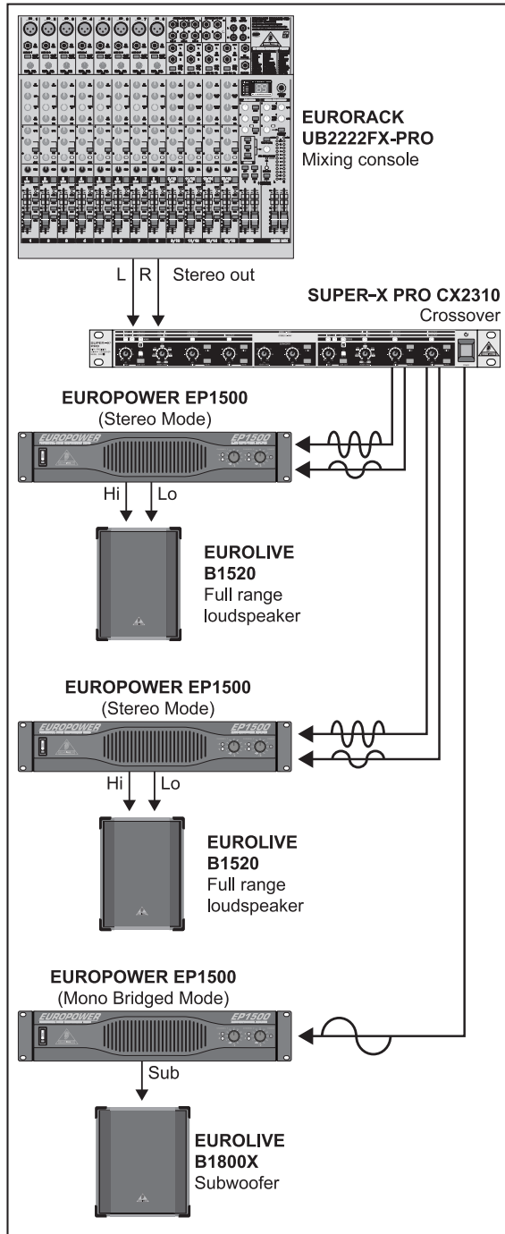
Fig. 3.7: Stereo bi-amp mode with a separate subwoofer
