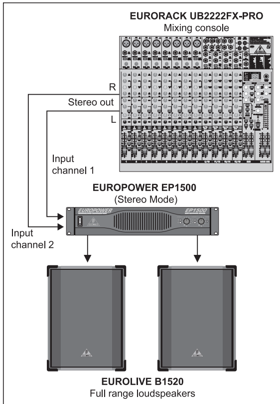
Fig. 3.1: 2-channel mode
