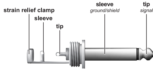
Fig. 4.4: 1/4" TS connector
