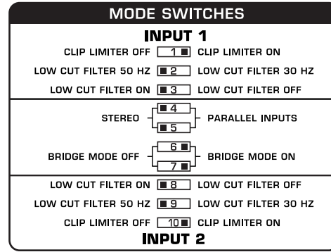
Fig. 3.6: DIP switch positions for mono-bridged mode
