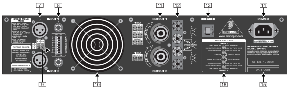
Fig. 2.2: Rear panel control elements
