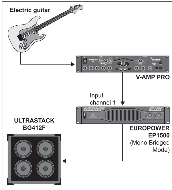
Fig. 3.5: Mono-bridged mode
