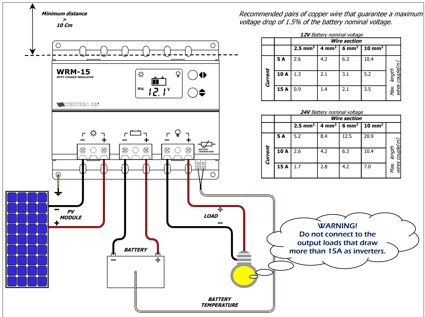
Fig. 2 Connection scheme
