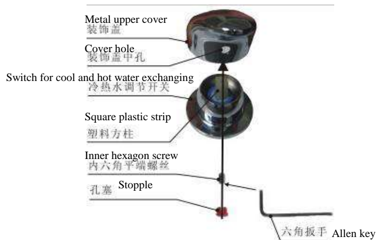
Installation Diagram of Switch A
