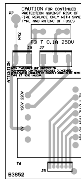
B3852 PCB
