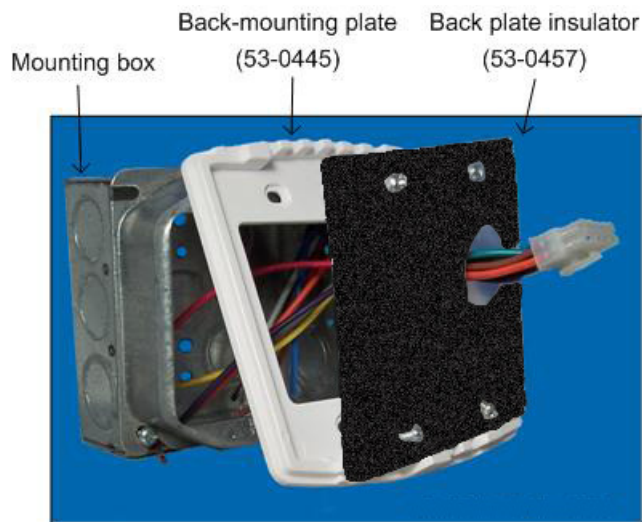
Figure 4 Mounting Assembly
