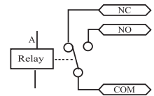
Relay Output Connection Diagram
