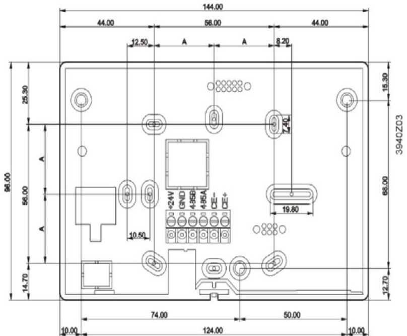
Figure 1: Physical Dimensions
