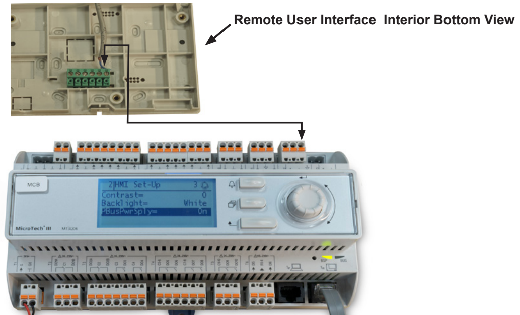
Figure 4: Interface Details for Daisy-Chain Connection
