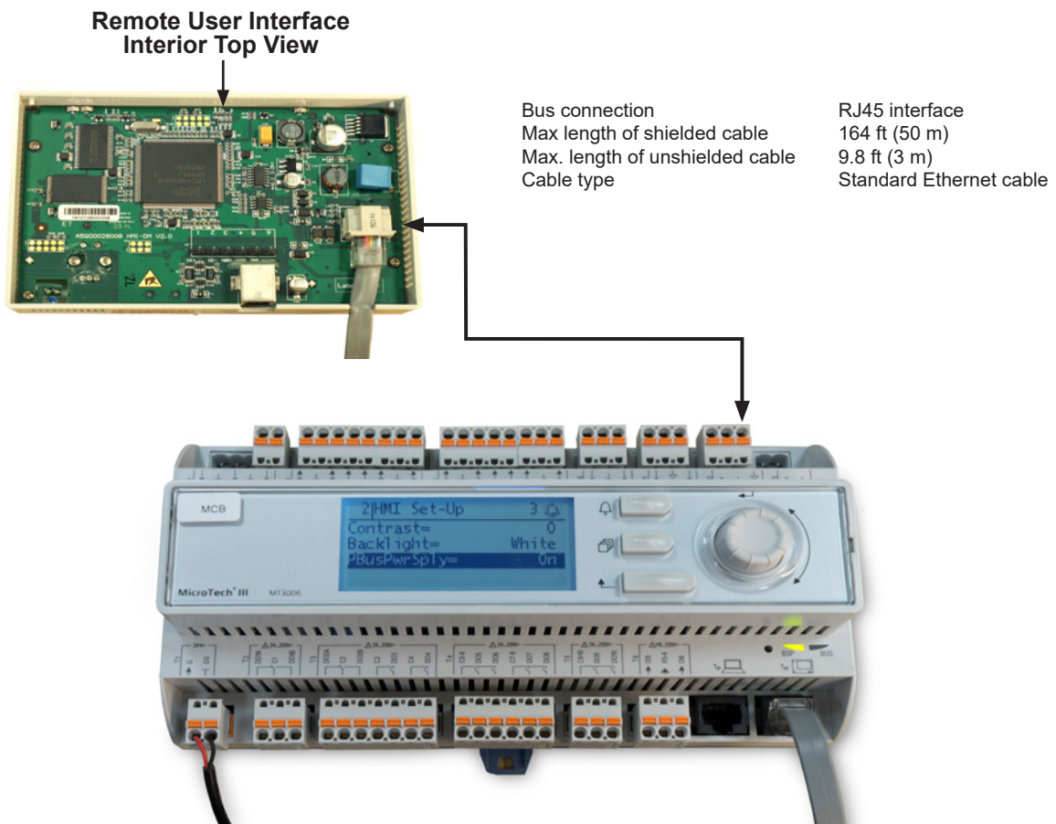
Figure 6: Interface Details for RJ45 Connector
