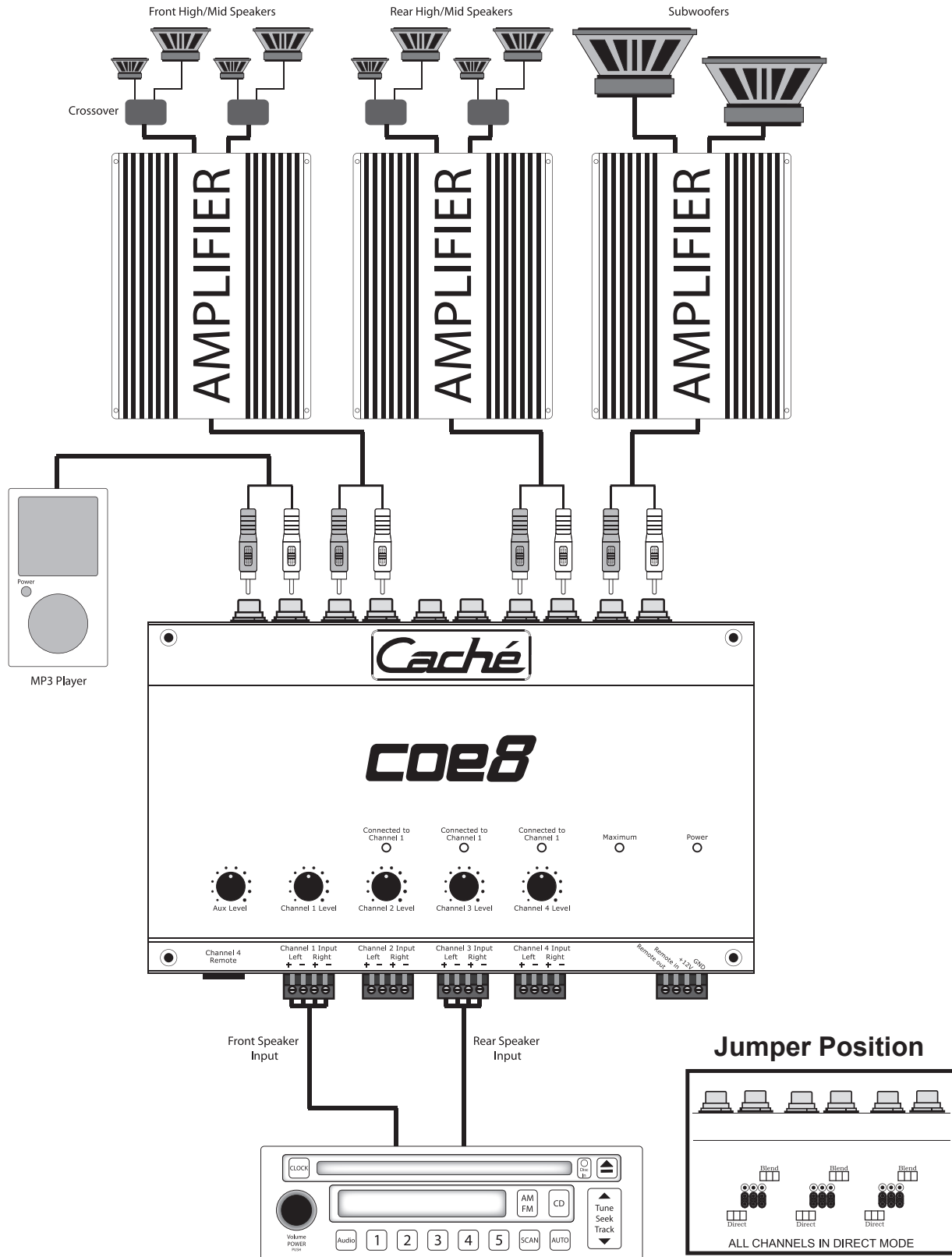
coe8 configuration for a full range high level 4 channel input system in direct mode.
